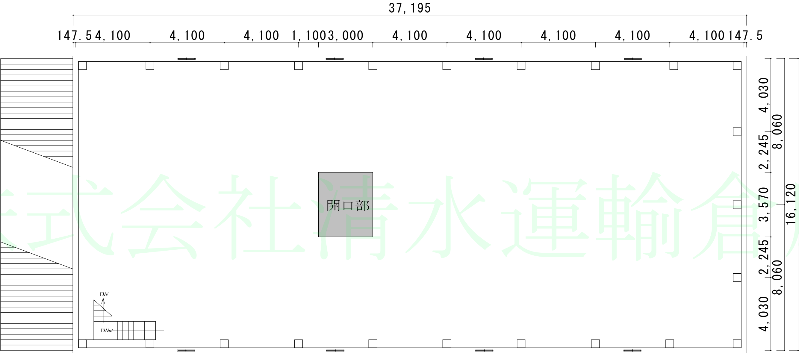
浮塚倉庫3号棟 2F S=1/100
